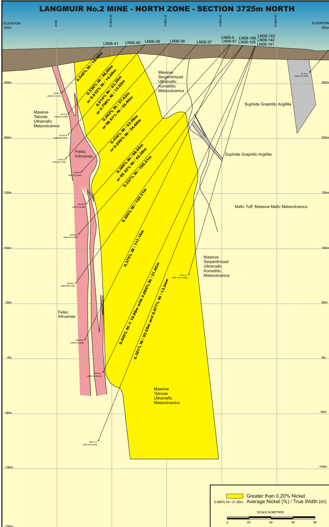
Figure 30: Typical Cross-Section at Langmuir No.2 Mine - North Zone.
