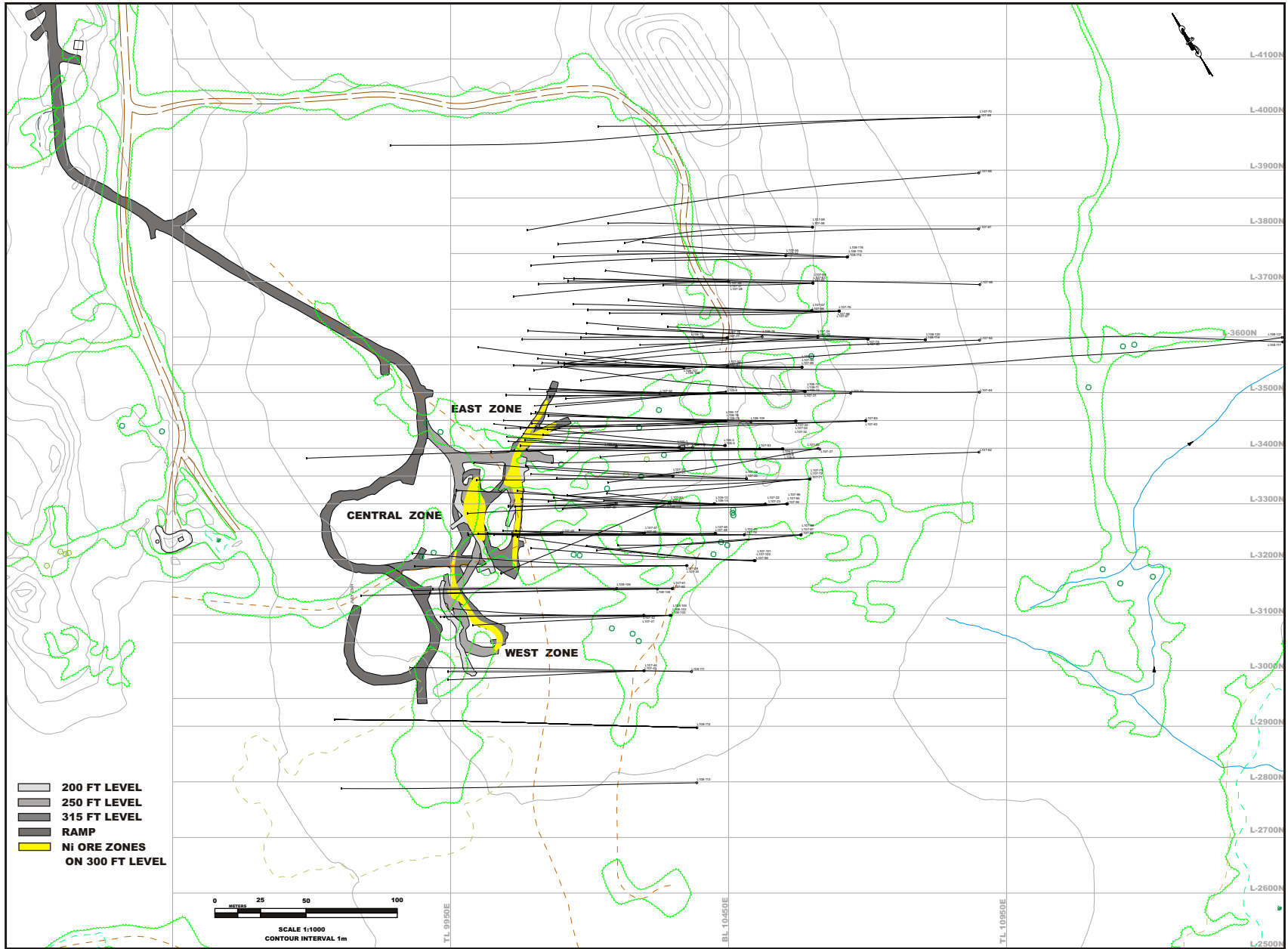
Figure 31: Diamond Drill Hole Location Map, Langmuir No.1 Mine.
