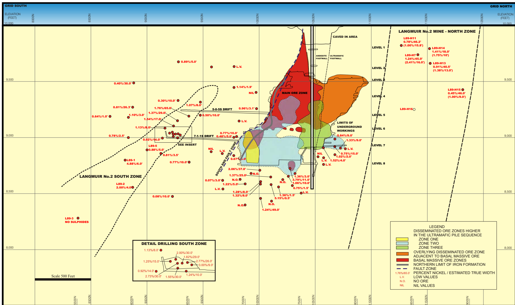
Figure 9: Langmuir No.2 Mine Vertical Longitudinal Looking Grid West or N303.5944E Astronomic. (modified after Timmins Nickel, February 1990 and MNDM Closure Plans)
