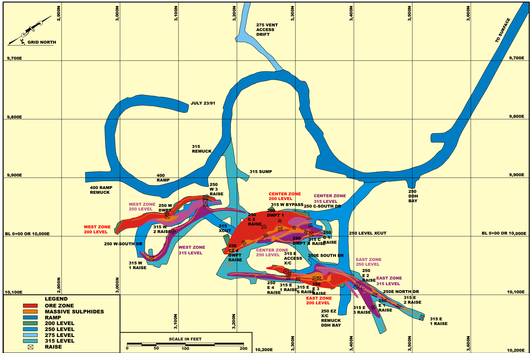
Figure 10: Langmuir No.1 Mine Underground Development and Ore Zones. (After Timmins Nickel, 1991)
