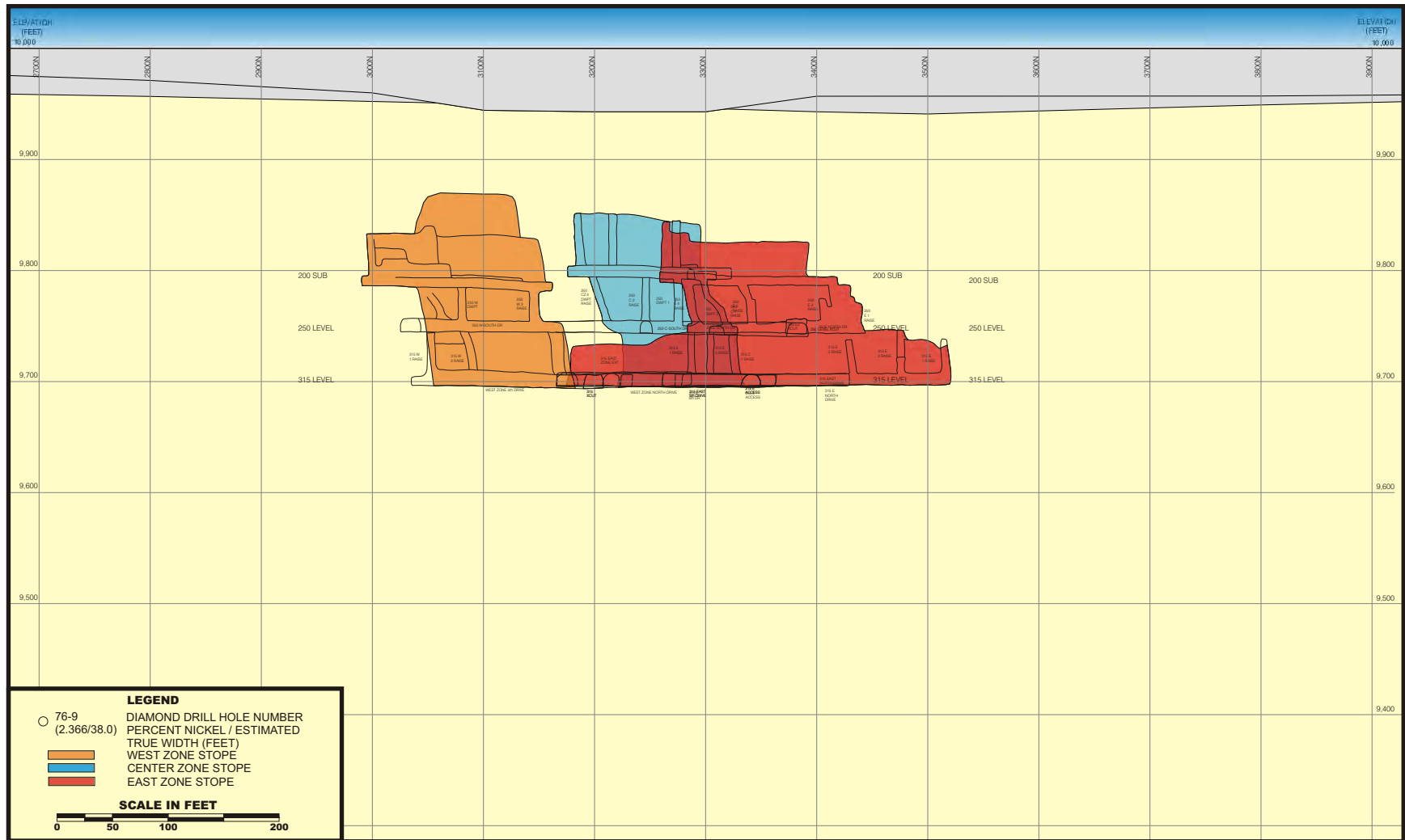
Figure 11: Langmuir No.1 Mine Composite Vertical Longitudinal, Looking Grid West. (Modified after Timmins Nickel)
