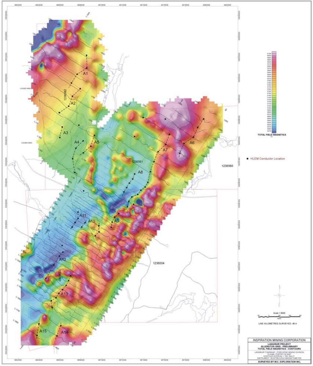
Figure 15: Shaded Total Field Magnetic Survey and Electromagnetic Conductors, Allerston Grid, Langmuir Property, Langmuir Township, Ontario. (Modified after Johnston, M., 2009)
