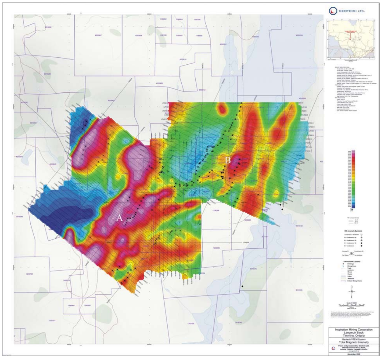
Figure 16: Airborne Total Field Magnetic Intensity with Electromagnetic VTEM Anomalies for the Langmuir Property (A = Langmuir No.1 Mine Zones, B = North Zone), Langmuir Township, Ontario.
