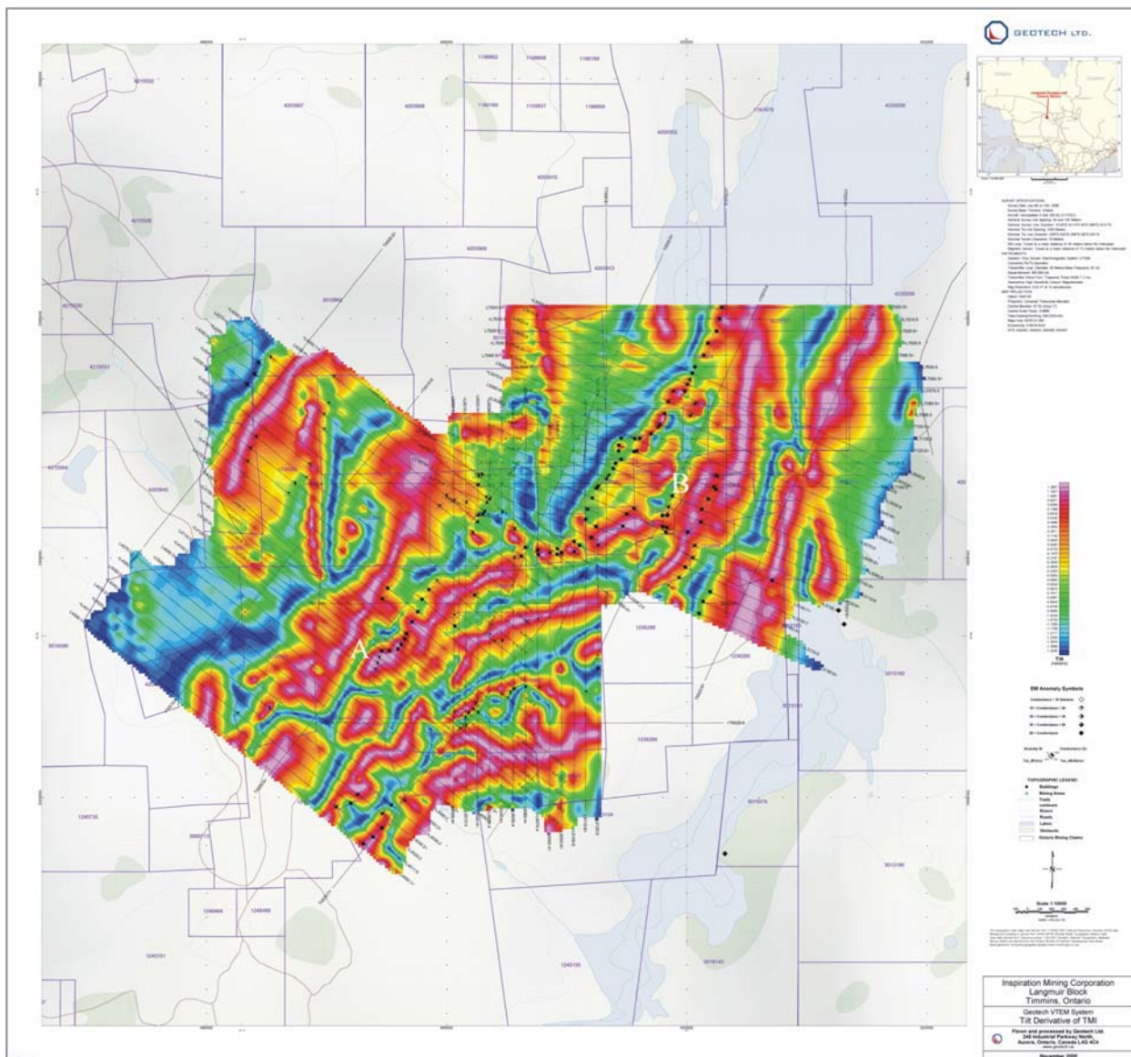
Figure 17: Tilt Derivative of the Total Field Magnetic Intensity with Electromagnetic VTEM Anomalies for the Langmuir Property (A = Langmuir No.1 Mine Zones, B = North Zone), Langmuir Township, Ontario.
